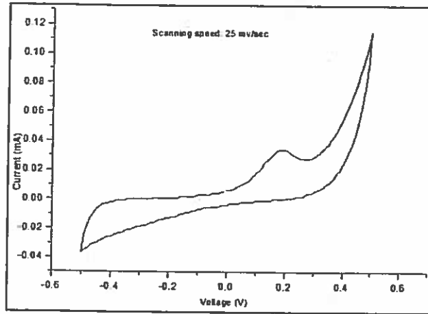
Fig.2 cyclic voltammetry of 0.1 N CdSO 4 , 0.1 N Na 2 S 2 O 3 and 0.1 N InCl 3 mixed electrolyte bath at scanning speed 25 mV/Sec
